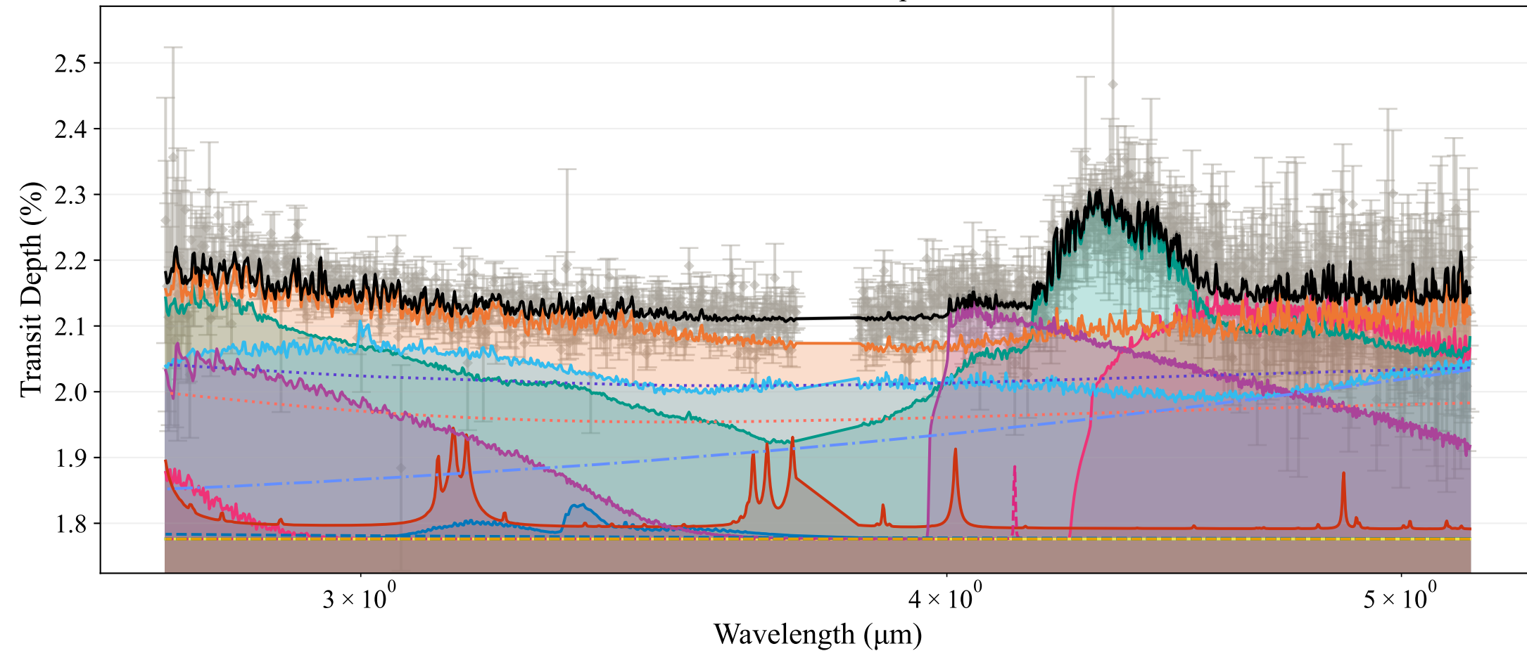
NIRSPEC, SiO, 4-point
